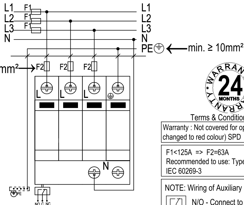
SPD MY3-65MAX (3P+N)
